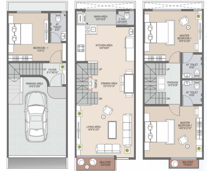
GROUND FLOOR LAYOUT FIRST FLOOR LAYOUT SECOND FLOOR LAYOUT
