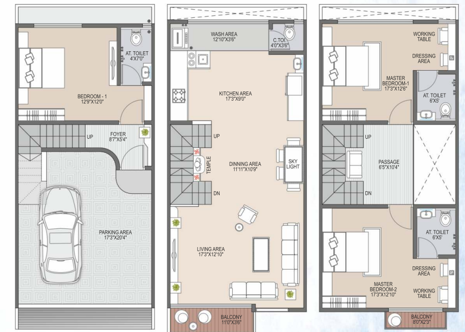
GROUND FLOOR LAYOUT FIRST FLOOR LAYOUT SECOND FLOOR LAYOUT
